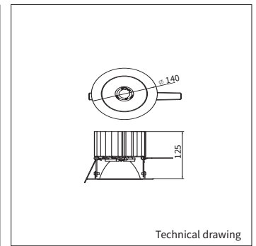
Technical drawing
